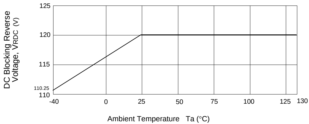
V_{R(DC)} - T_a Characteristic
