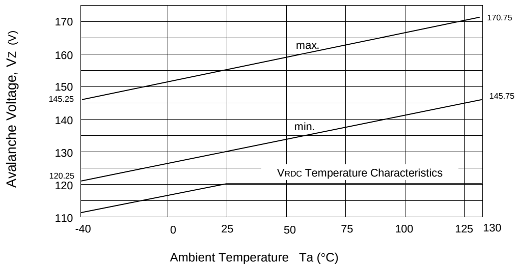
V_Z Temperature Coefficient
