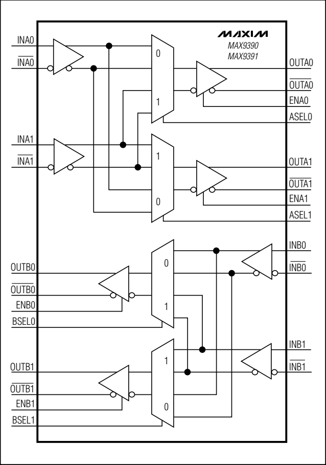
Functional Diagram
