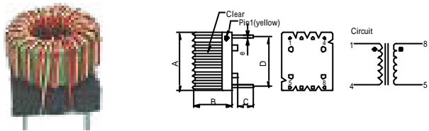
BCB1306RI-221-N
