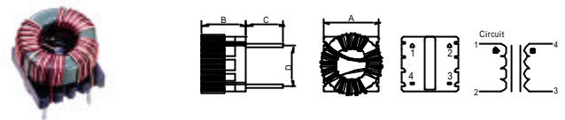
BCB1306RI-221-N
