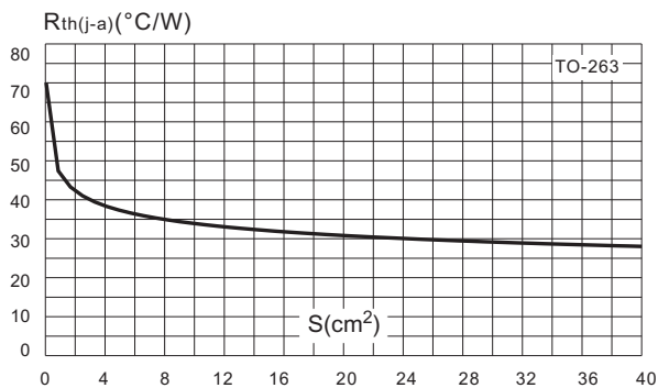
Fig.11 D 2 PAK thermal resistance junction to ambient versus copper surface under tab (printed circuit board FR4, copper thickness: 35 \mu\text{m} )
