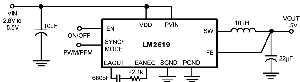
FIGURE 3. Typical Circuit for 1.5V Output Voltage
