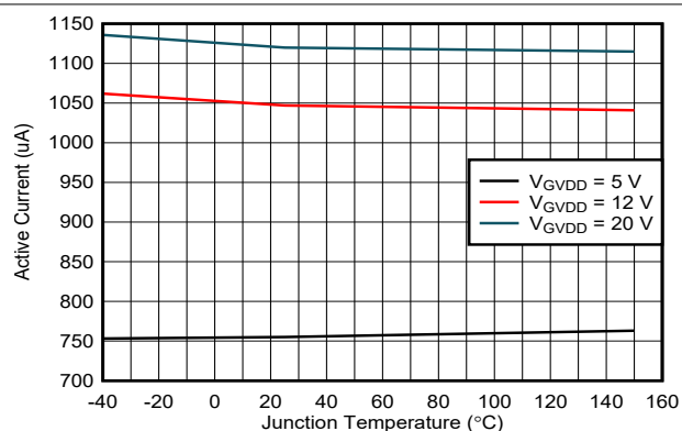
Figure 7-4. Supply Current Over Temperature
