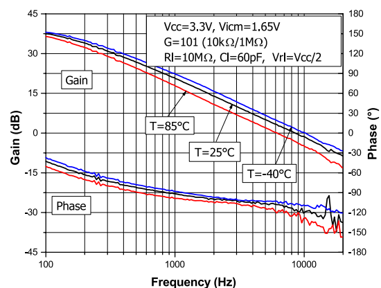
Figure 25: Bode diagram at 3.3 V supply voltage
