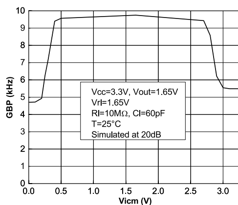
Figure 27: Gain bandwidth product vs. input common-mode voltage
