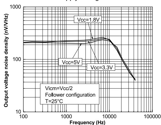
Figure 29: Noise vs. frequency for different power supply voltages
