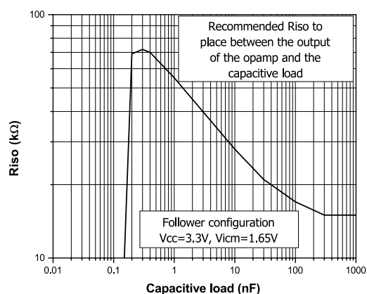
Figure 28: In-series resistor (Riso) vs. capacitive load
