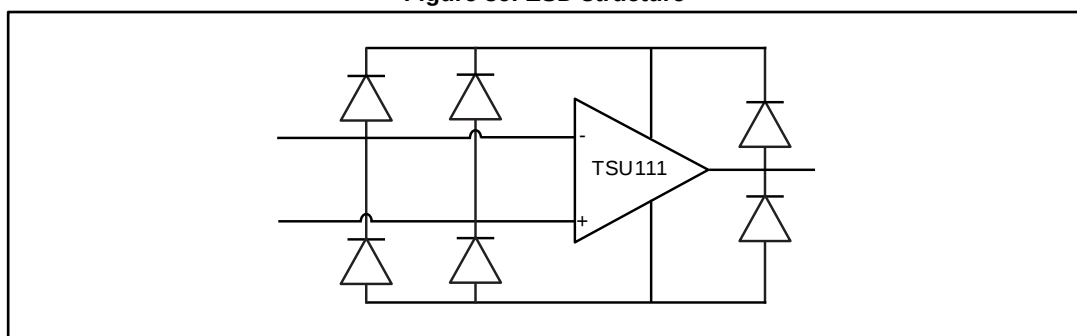
Figure 36: ESD structure
