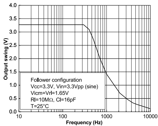
Figure 18: Output swing vs. input signal frequency
