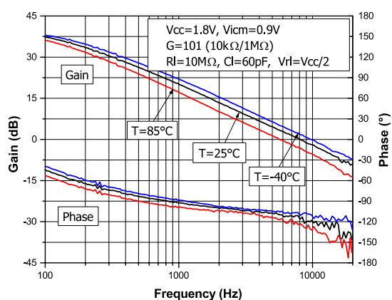
Figure 24: Bode diagram at 1.8 V supply voltage
