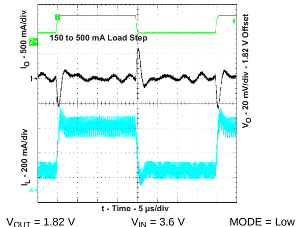
Figure 19. Load Transient Response in PFM/PWM Operation, V_{OUT} = 1.82\text{ V} , V_{IN} = 3.6\text{ V}
