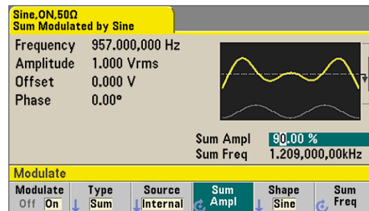
Dual-tone signal created by summing waveforms using the modulation type, "Sum."
