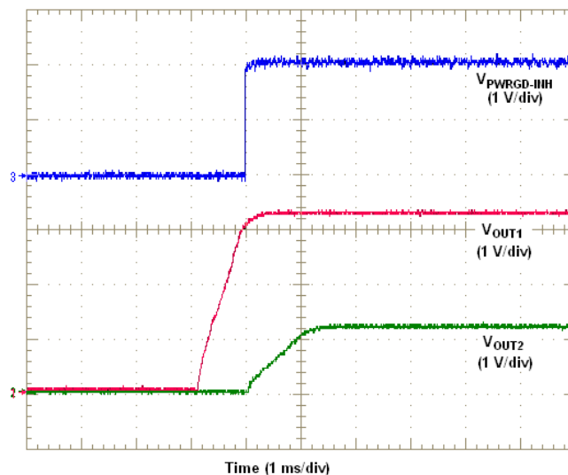
Figure 30. Sequencing Waveforms
