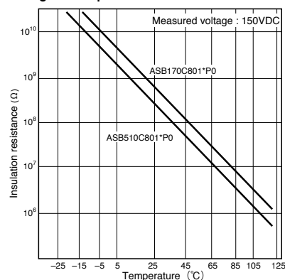
Fig-15 Temperature vs. Insulation resistance
