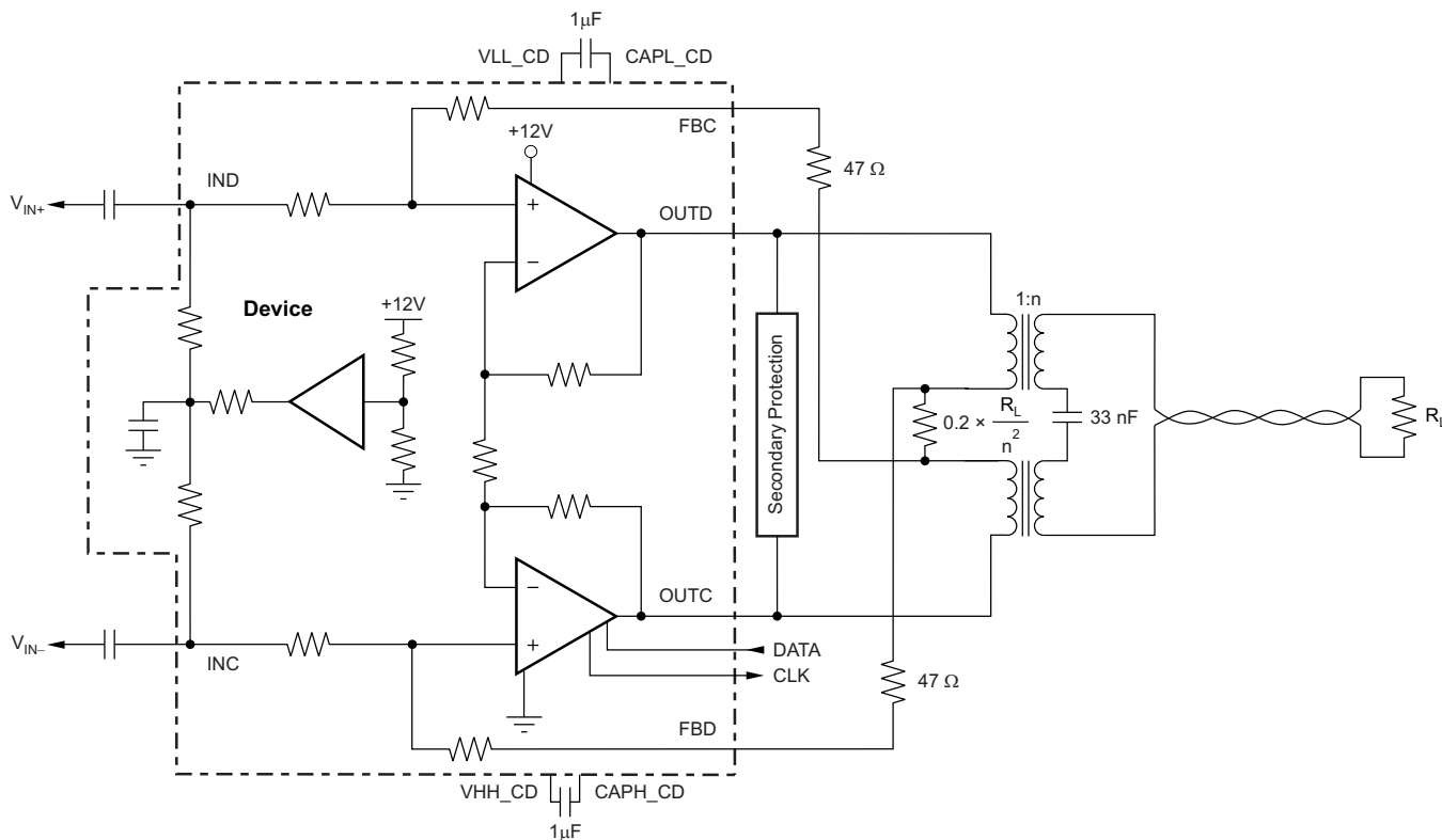
Figure 34. Typical VDSL Line Driver Circuit Configuration
