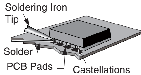
Figure 35: Soldering Technique
