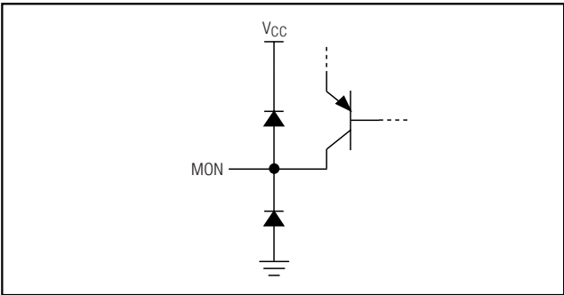
Figure 8. MON Interface
