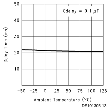
Reset Delay Time vs Temperature
