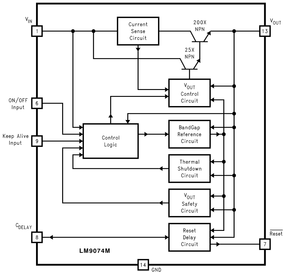
Block Diagram
