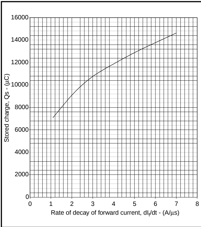
Fig. 4 Stored charge
