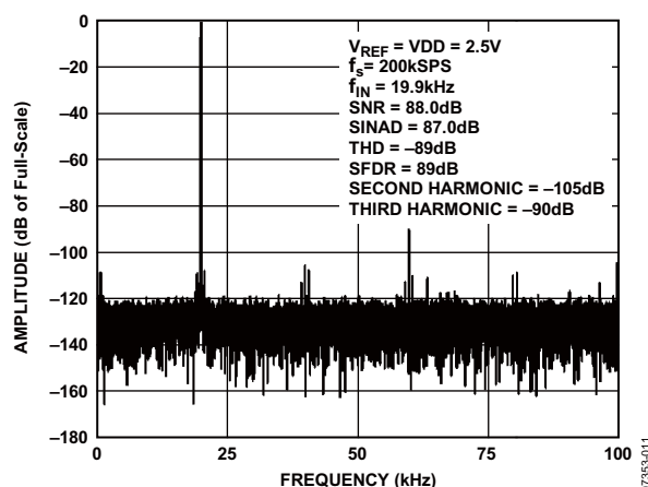
图11. 20 kHz FFT, V_{REF} = V_{DD} = 2.5\text{ V}
