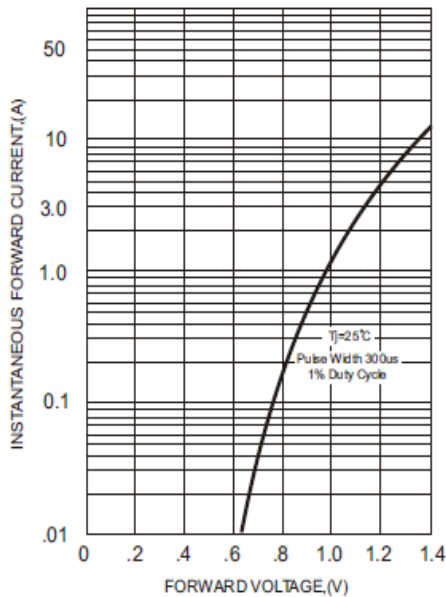
FIG.3-TYPICAL FORWARD CHARACTERISTICS
