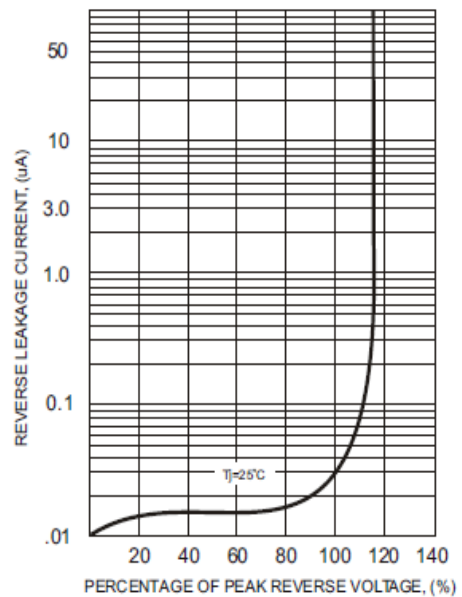
FIG.4-TYPICAL REVERSE CHARACTERISTICS
