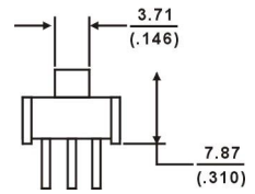
TSR-3386(STYLE)-EY5-(RESISTANCE CODE)-T
