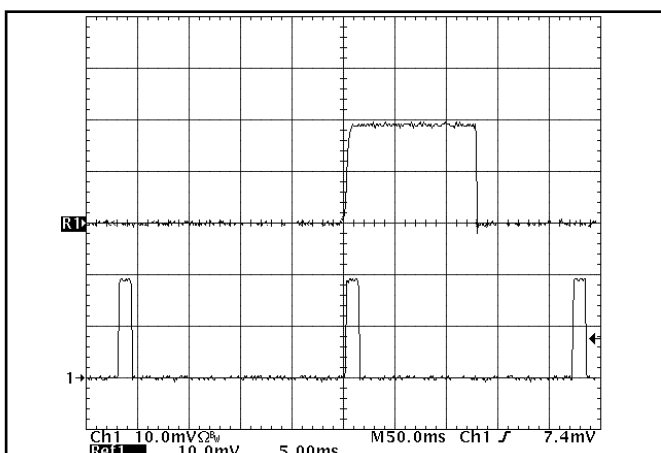
Figure 18: Load current (10A/div) as a function of time when the converter attempts to turn on into a 10 m \Omega short circuit. Top trace (5.0ms/div) is an expansion of the on-time portion of the bottom trace.
