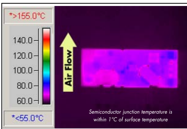
Figure 6: Thermal plot of converter at 15 amp load current with 55°C air flowing at the rate of 200 LFM. Air is flowing across the converter from pin 3 to pin 1 (nominal input voltage).
