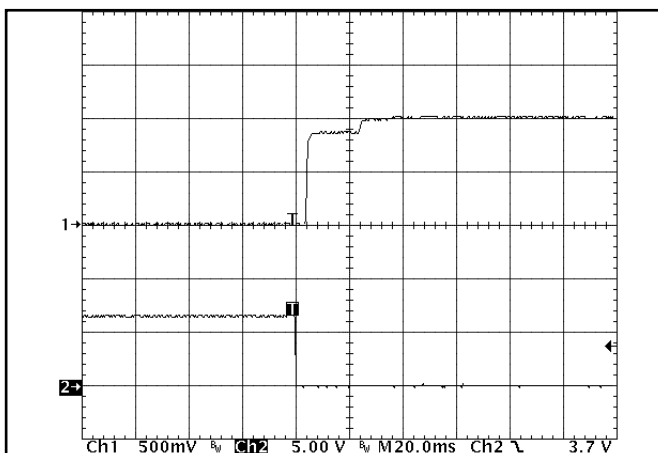
Figure 10: Turn-on transient at zero load (20 ms/div). Ch 1: V_{out} (500mV/div). Ch 2: ON/OFF input (5V/div)
