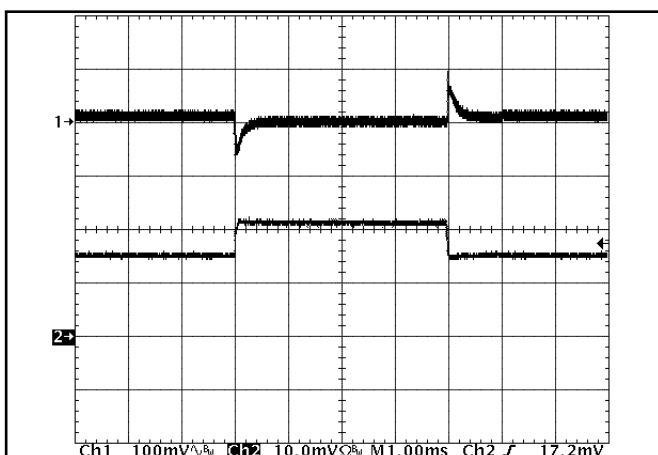
Figure 12: Output voltage response to step-change in load current (50%-75%-50% of I_{out(max)} ; dI/dt = 5A/\mu s ). Load cap: 470 \mu F, 30 m \Omega ESR tantalum capacitor and 1 \mu F ceramic cap. Ch 1: V_{out} (100mV/div), Ch 2: I_{out} (5A/div).
