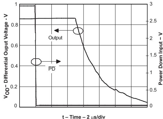
Figure 69. Turnoff Time
