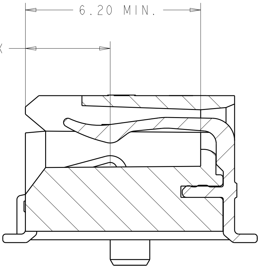
SECTION X-X
