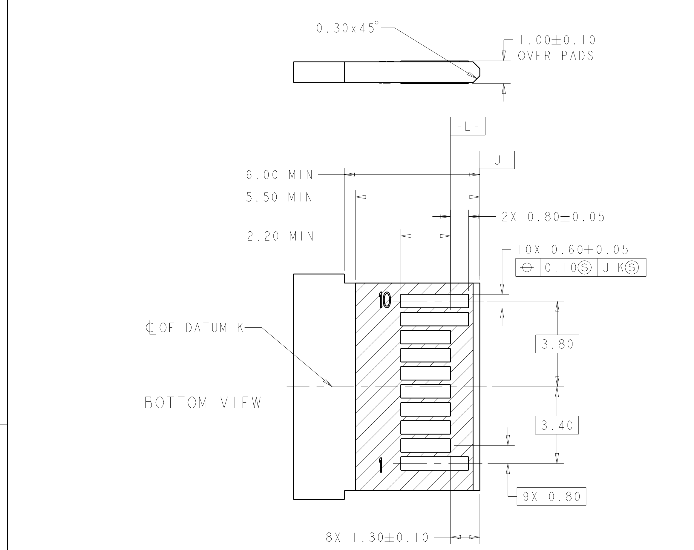
RECOMMENDED LAYOUT DETAIL MATING TRANSCEIVER PCB SCALE 10:1
