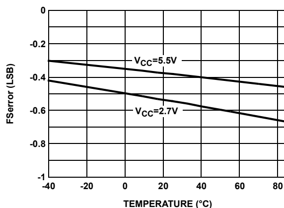
FIGURE 6. FSerror vs TEMPERATURE FOR 50k \Omega (W)
