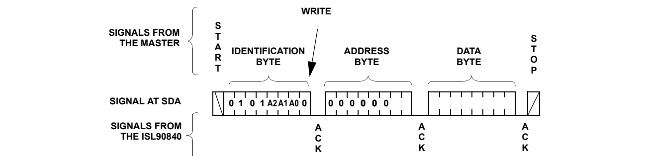
FIGURE 17. BYTE WRITE SEQUENCE
