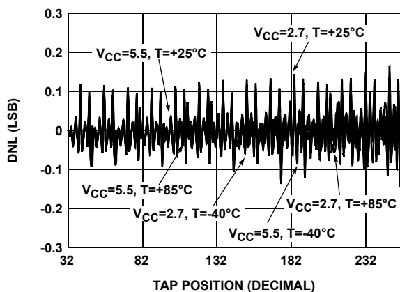
FIGURE 7. DNL vs TAP POSITION IN RHEOSTAT MODE FOR 50k \Omega (U)
