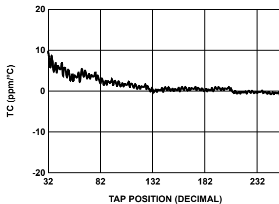
FIGURE 10. TC FOR VOLTAGE DIVIDER MODE IN ppm FOR 50k \Omega (W)
