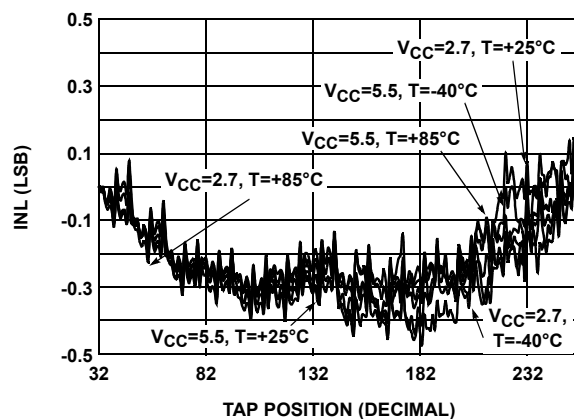
FIGURE 8. INL vs TAP POSITION IN RHEOSTAT MODE FOR 50k \Omega (U)
