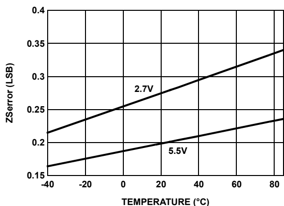
FIGURE 5. ZSerror vs TEMPERATURE FOR 50k \Omega (W)
