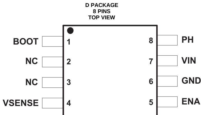
Pin Functions
