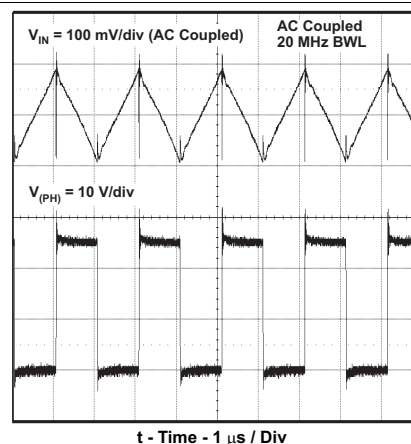
Figure 13. Input Voltage Ripple and PH Node, I_O = 1\text{ A}
