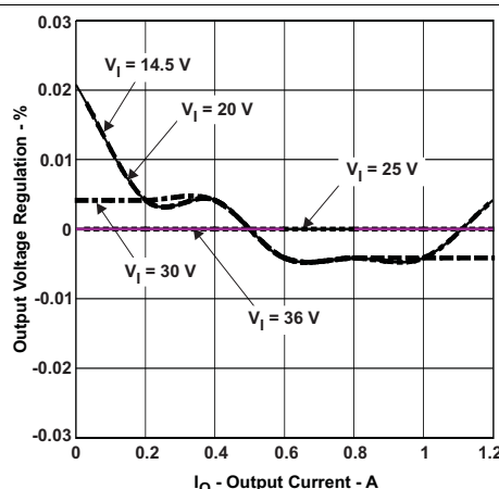
Figure 11. Output Voltage Regulation % vs. Output Current
