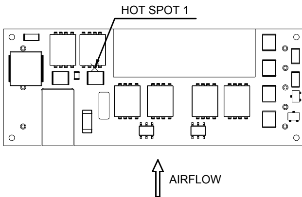
Figure 21: * Hot spot 1 & NTC resistor temperature measured points. The allowed maximum hot spot 1 temperature is defined at 124
