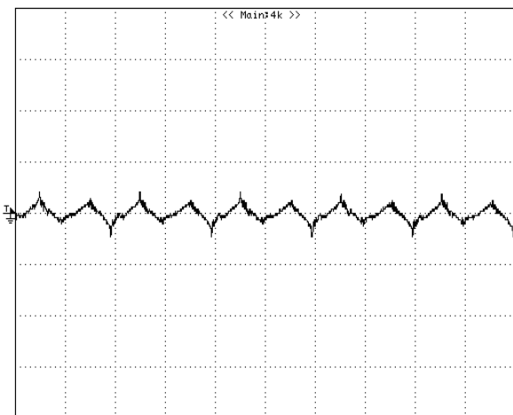
Figure 14: Output voltage ripple at nominal input voltage and rated load current ( I_o=30\text{A} ) (50 mV/div, 2us/div) Load capacitance: 1\mu\text{F} ceramic capacitor and 10\mu\text{F} tantalum capacitor. Bandwidth: 20 MHz. Scope measurements should be made using a BNC cable (length shorter than 20 inches). Position the load between 51 mm to 76 mm (2 inches to 3 inches) from the module.
