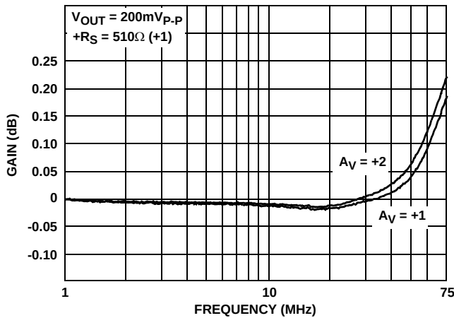
FIGURE 19. GAIN FLATNESS
