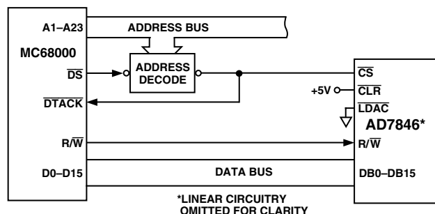
Figure 25. AD7846-to-MC68000 Interface
