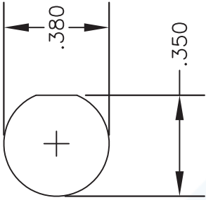
MOUNTING HOLE
