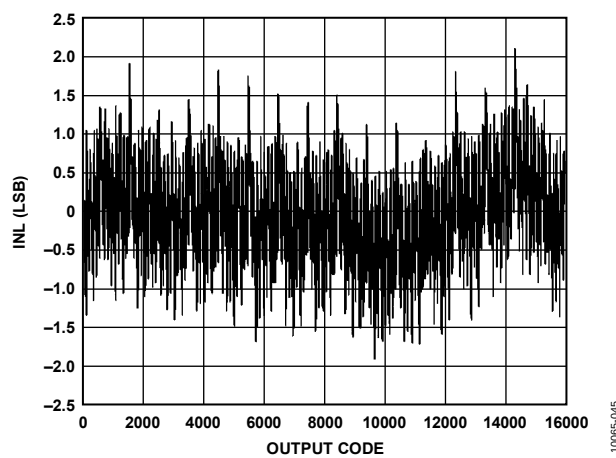
Figure 41. INL, f_{IN} = 9.7 MHz, f_{SAMPLE} = 125 MSPS
