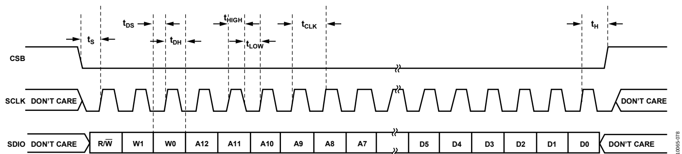
Figure 74. Serial Port Interface Timing Diagram
