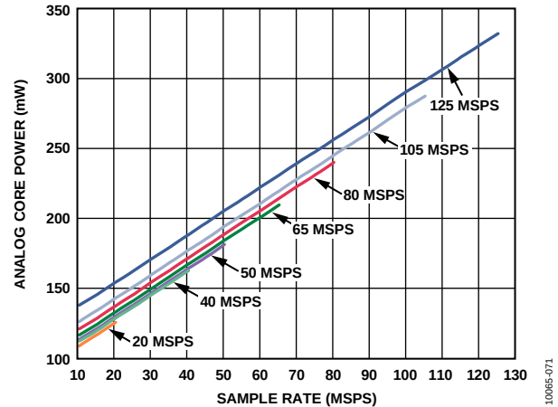
Figure 69. Analog Core Power vs. f_{\text{SAMPLE}} for f_{\text{IN}} = 10.3 \text{ MHz}
