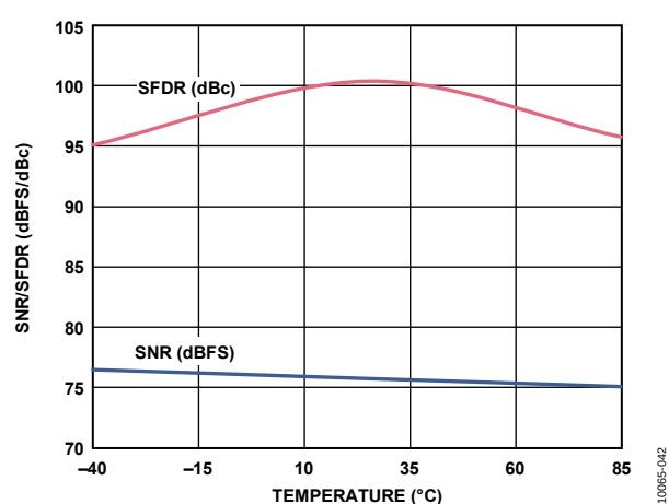
Figure 19. SNR/SFDR vs. Temperature, f_{IN} = 10.3 MHz, f_{SAMPLE} = 80 MSPS
