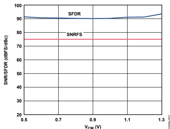
Figure 56. SNR/SFDR vs. Common-Mode Voltage, f_{IN} = 9.7 \text{ MHz} , f_{SAMPLE} = 125 \text{ MSPS}
