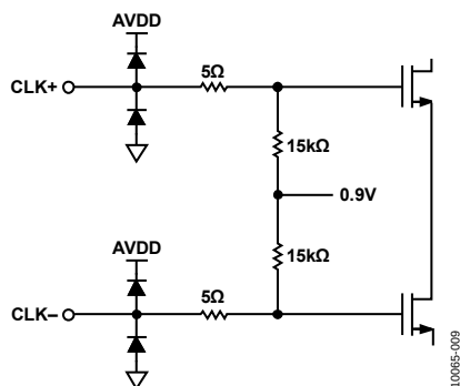
Figure 48. Equivalent Clock Input Circuit
