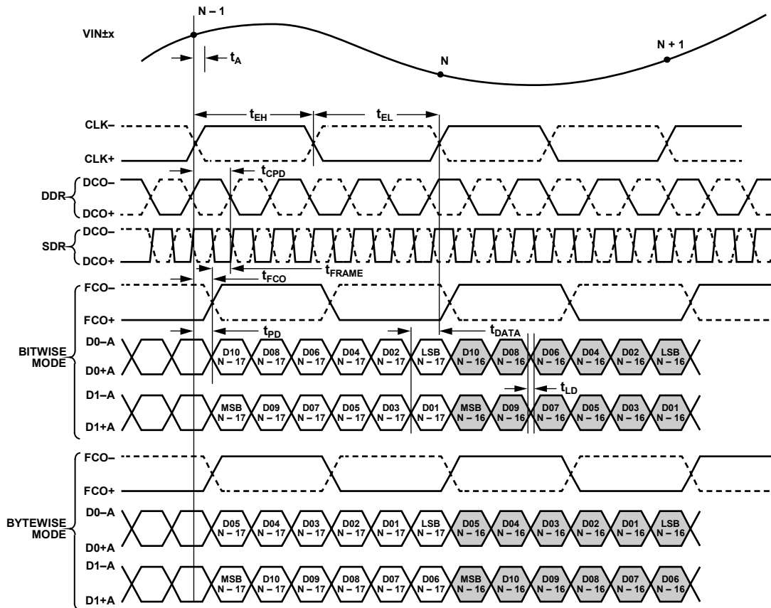
Figure 3. 12-Bit DDR/SDR, Two-Lane, 1x Frame Mode
