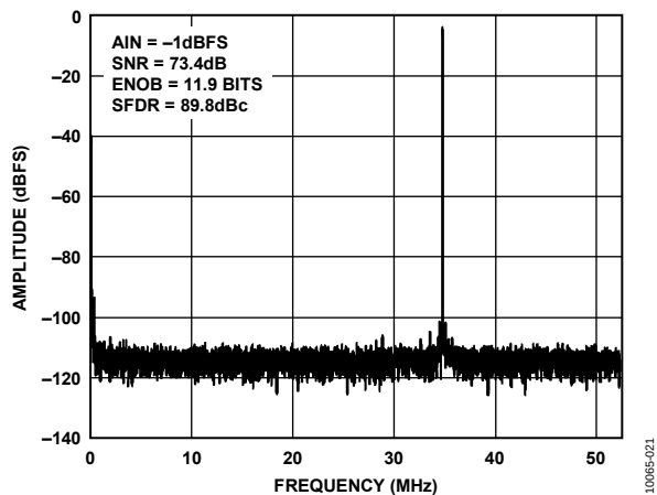
Figure 22. Single-Tone 16k FFT with f_{IN} = 70 MHz, f_{SAMPLE} = 105 MSPS
