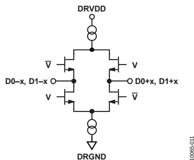
Figure 50. Equivalent Digital Output Circuit
