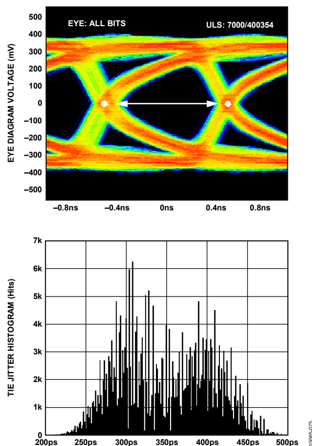
Figure 72. Data Eye for LVDS Outputs in ANSI-644 Mode with Trace Lengths Less than 24 Inches on Standard FR-4 Material, External 100 \Omega Far-End Termination Only
