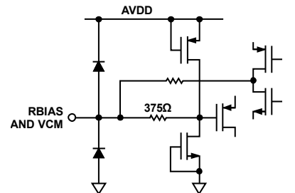
Figure 52. Equivalent RBIAS and VCM Circuit
