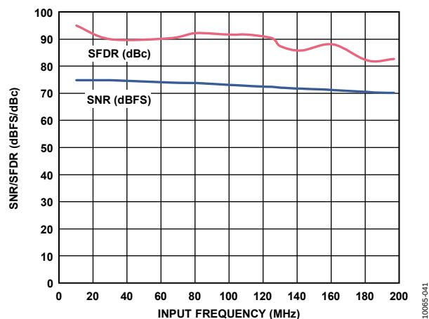
Figure 39. SNR/SFDR vs. f_{IN} , f_{SAMPLE} = 125 MSPS
