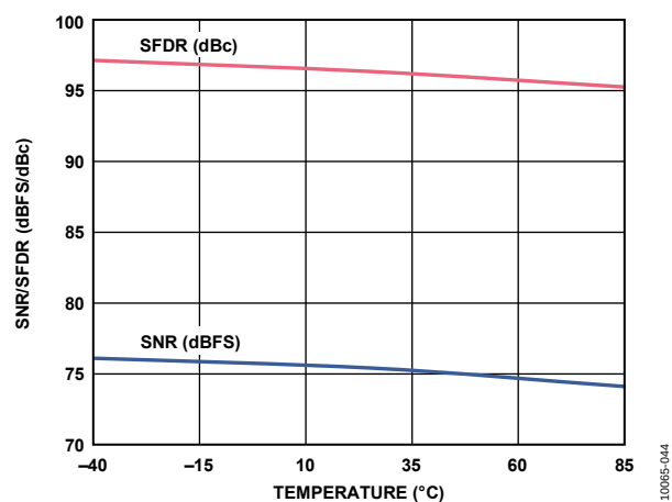
Figure 40. SNR/SFDR vs. Temperature, f_{IN} = 10.3 MHz, f_{SAMPLE} = 125 MSPS
