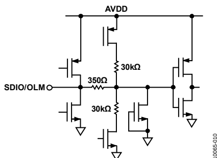
Figure 49. Equivalent SDIO/OLM Input Circuit
