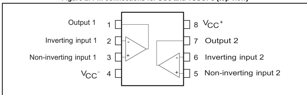
Figure 2: Pin connections for SO8 and TSSOP8 (top view)
