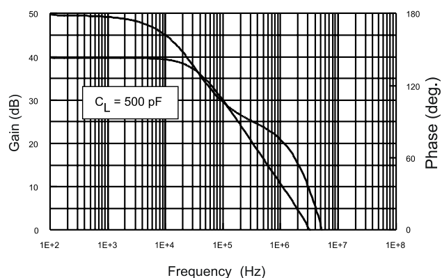
Figure 13: Open loop gain and phase vs. frequency
