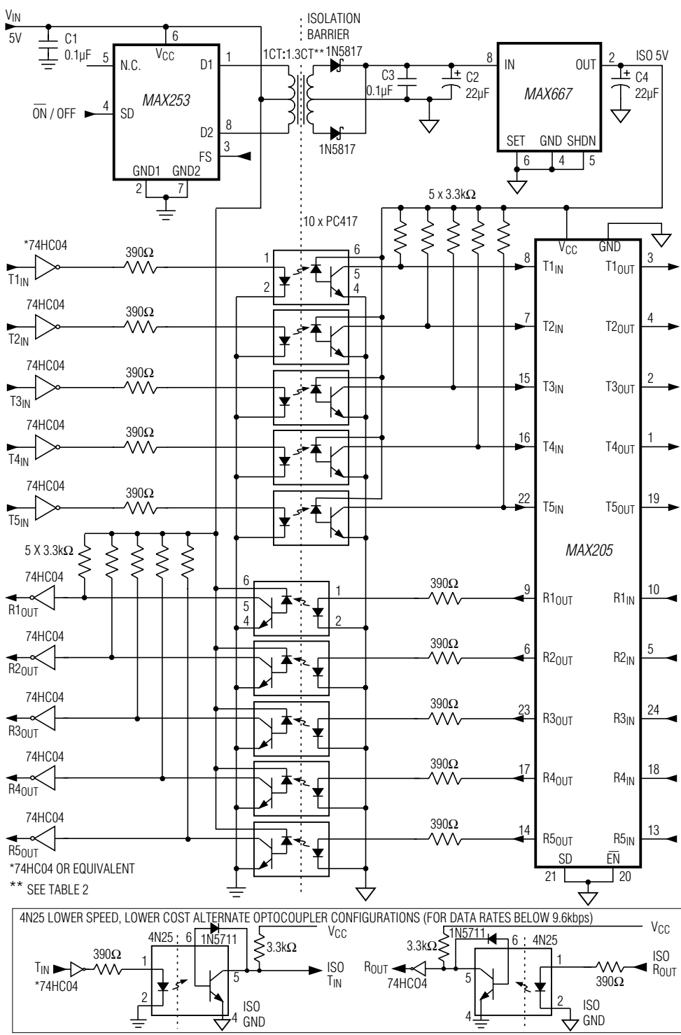
Figure 5. Typical RS-232 Application Circuit
