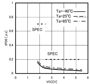
Fig.25 Data "0" output delay time tPD0
