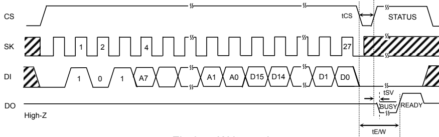
Fig.34 Write cycle
