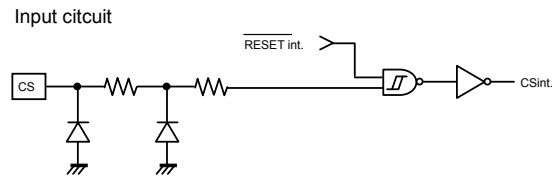
Fig.41 Input circuit (CS)
