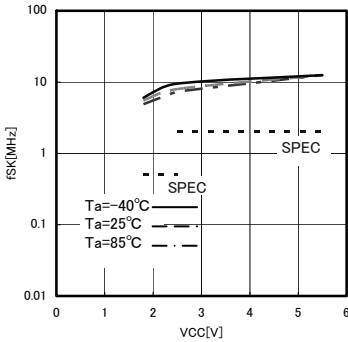
Fig.17 SK frequency fSK
