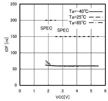
Fig.28 Time from CS to High-Z tDF
