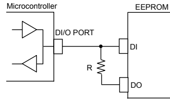
Fig.49 DI, DO control line common connection
