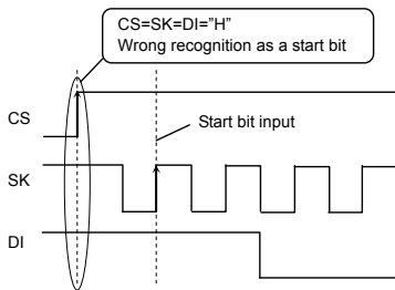
Fig.38 Wrong action timing
