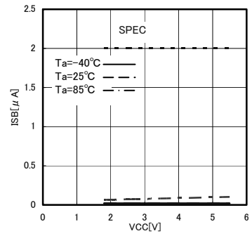
Fig.16 Consumption current at standby action ISB
