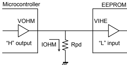
Fig.44 CS pull down resistance
