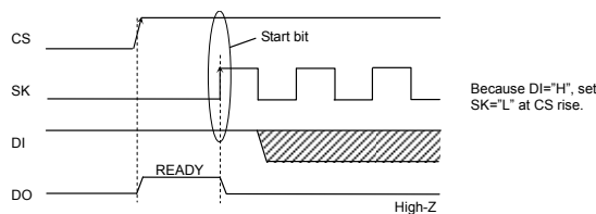
Fig.52 Start bit input timing at DI, DO direct connection
