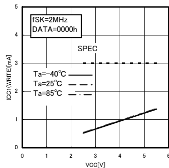
Fig.12 Current consumption at WRITE action ICC1(WRITE, fSK=2MHz)
