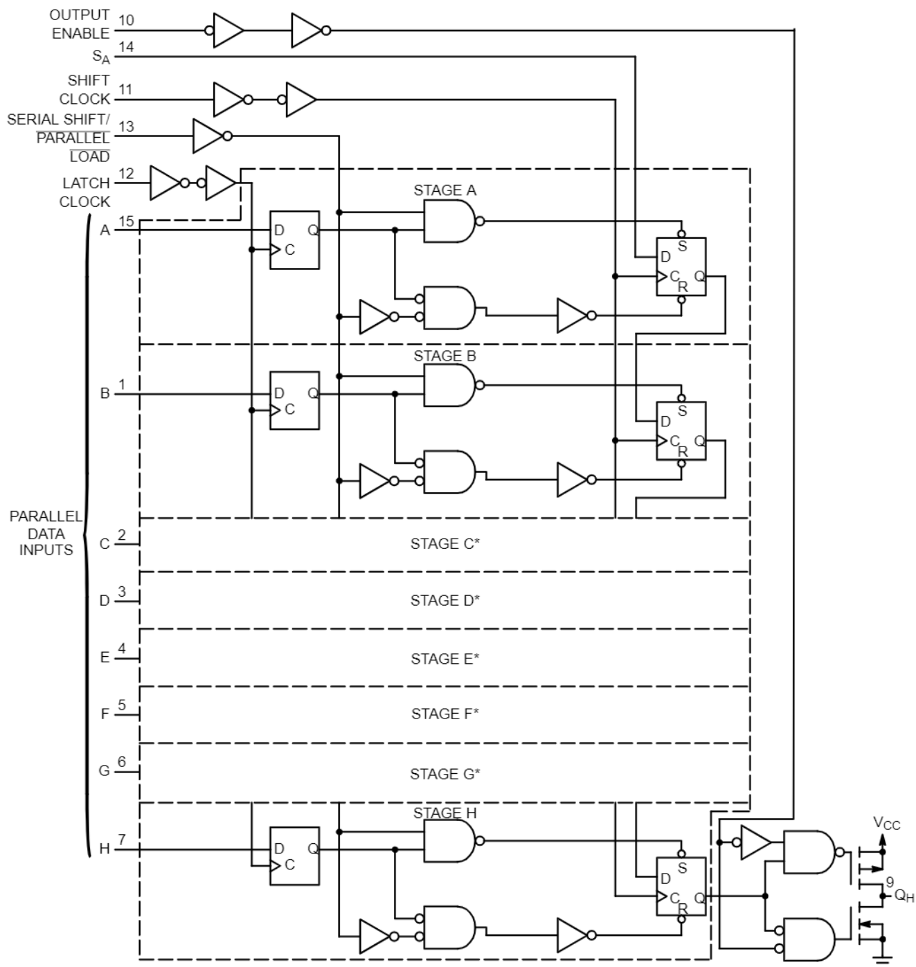
Figure 12. Logic Detail
