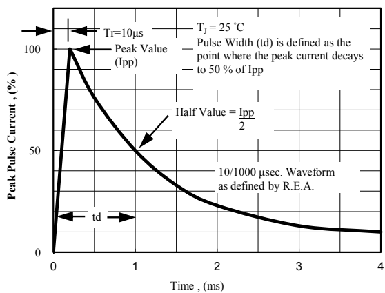
Fig. 5 - Pulse Waveform
