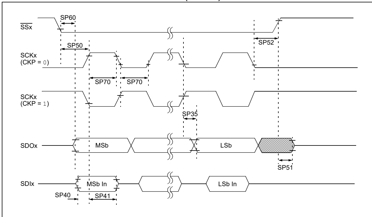
FIGURE 33-13: SPIx MODULE SLAVE MODE (CKE = 1) TIMING CHARACTERISTICS
