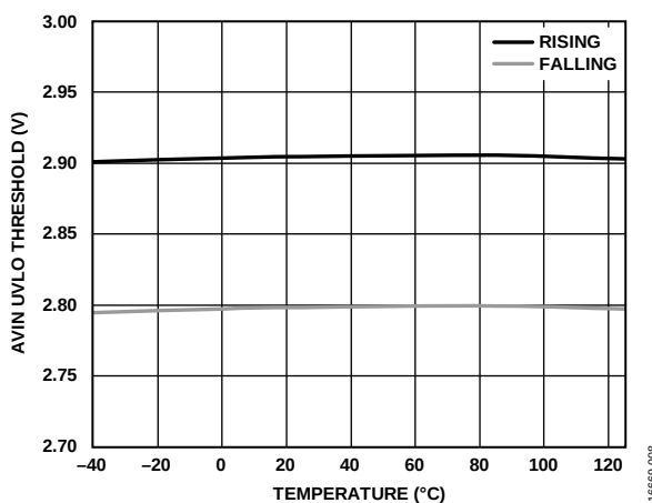
Figure 8. AVIN UVLO Threshold vs. Temperature
