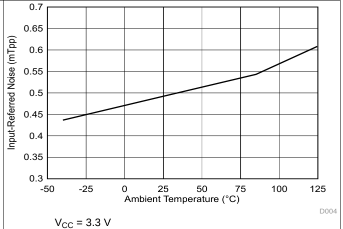
Figure 6. B_N vs Temperature
