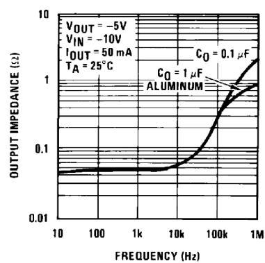
Output Impedance
