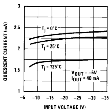
Quiescent Current
