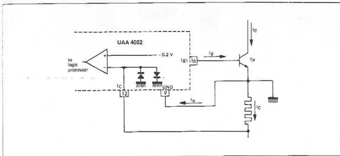
Figure 3 : Switching Transistor Collector Current Measurement.
