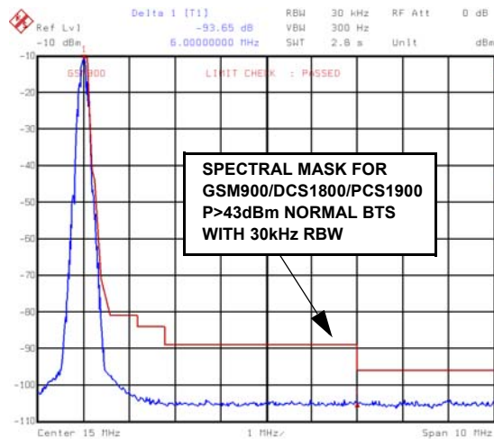
FIGURE 3. GSM AT 11MHz, 78MSPS CLOCK (94+dBc @ \Delta f = +6 MHz, 3dB PAD)
