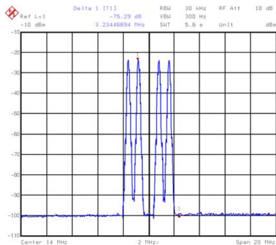
FIGURE 5. FOUR EDGE CARRIERS AT 12.4-15.6MHz, 800kHz SPACING, 78MSPS (75+dBc - 20MHz WINDOW)
