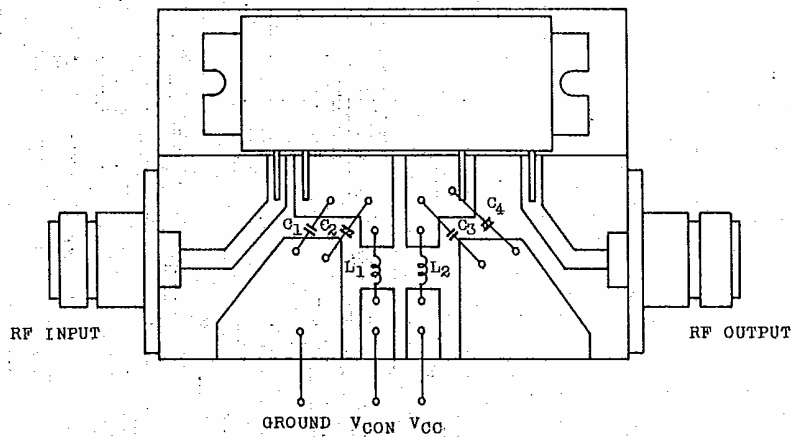
TEST MOUNT
