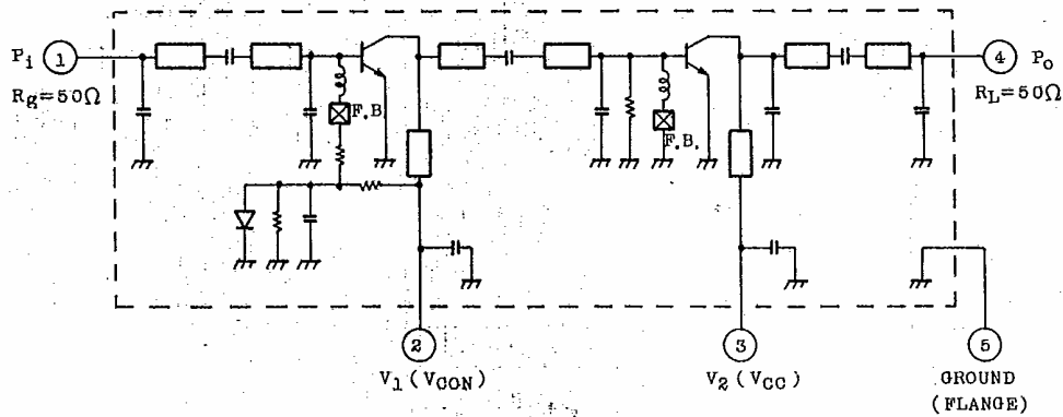
SCHEMATIC
