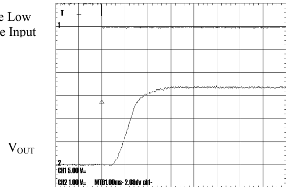
Turn-On with 47 \Omega /150 \mu F Load
