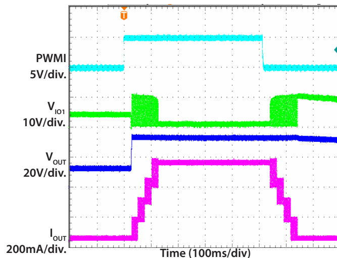
LED Open Circuit Protection
