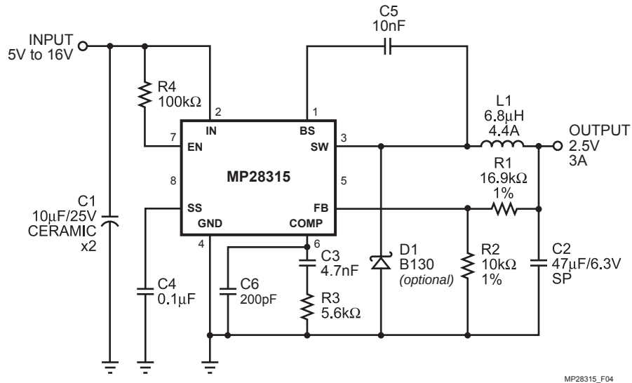
Figure 4—MP28315 with Panasonic 47μF, 6.3V Solid Polymer Output Capacitor
