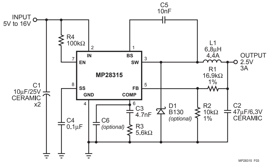
Figure 3—MP28315 with AVX 47μF, 6.3V Ceramic Output Capacitor
