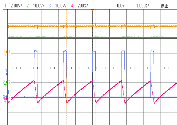
Switching waveform Vin=3.6V, 10 LEDs
