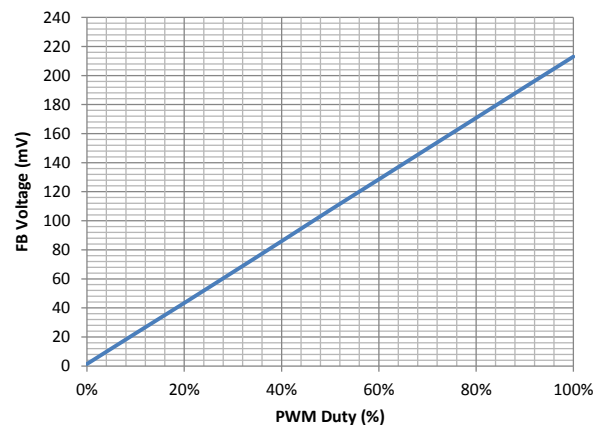
FB Voltage Vs. PWM Duty Cycle
