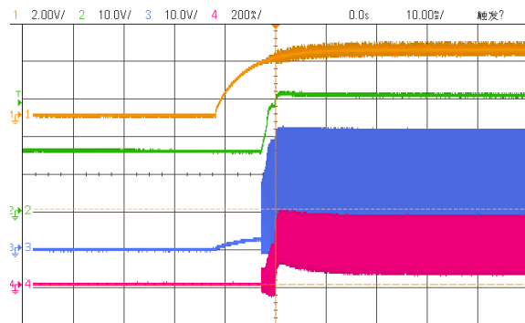
Startup waveform Vin=3.6V, 10 LEDs (CH1=Vin, CH2=Vout, CH3=SW, CH4=Isw)
