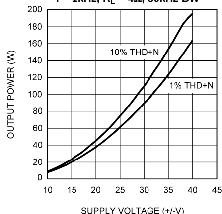
Output Power vs Supply Voltage, Parallel Mode f = 1kHz , R_L = 4\Omega , 80kHz BW
