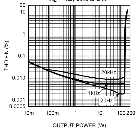
THD+N vs Output Power \pm 35V , Parallel Mode R_L = 4\Omega , 80kHz BW
