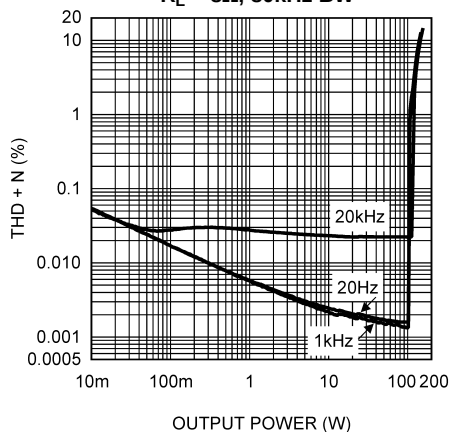
THD+N vs Output Power \pm 25V , Bridge Mode R_L = 8\Omega , 80kHz BW
