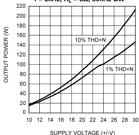
Output Power vs Supply Voltage, Bridge Mode f = 1kHz , R_L = 8\Omega , 80kHz BW
