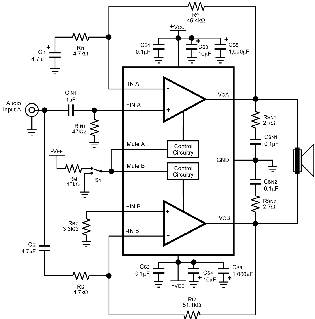
Figure 3. Bridged Amplifier Application Circuit
