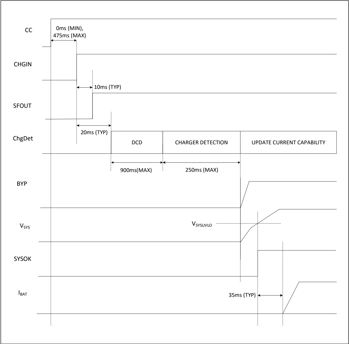
Figure 3b. Type-C Adapter Insertion ( CHGINILimGate = 1 )
