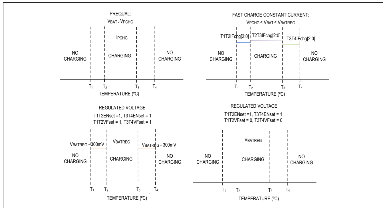
Figure 6. Thermistor Monitoring
