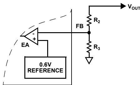
FIGURE 58. EXTERNAL RESISTOR DIVIDER
