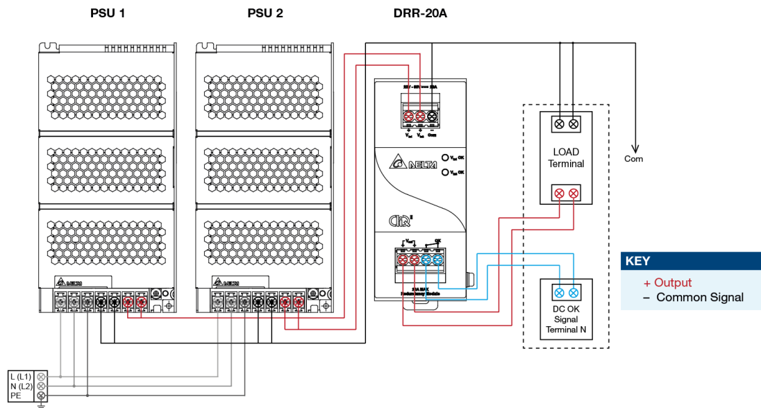
Fig. 3 Redundancy / Parallel Operation Connection Diagram
