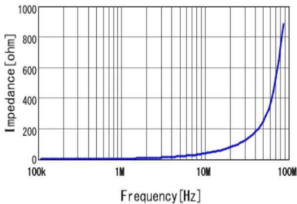
■DFE201610P-R68M |Z|
